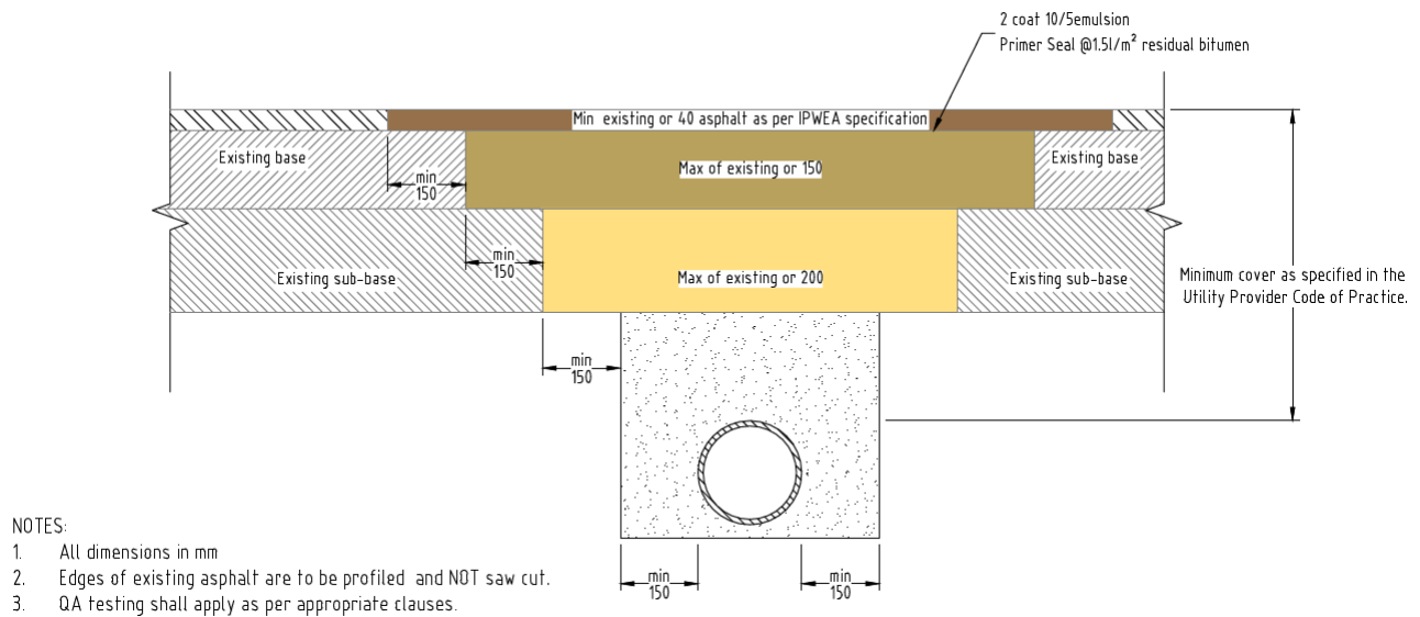
Figure 8-1: Typical cross section for reinstatement of trenches
